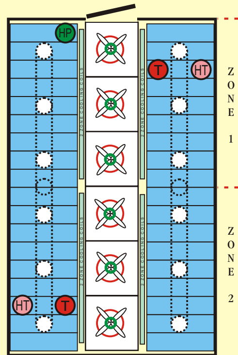
C576-165 Classic Setter Internal Layout
